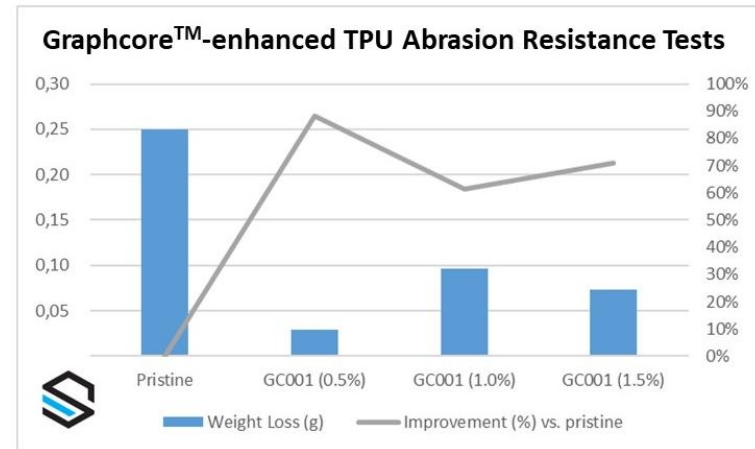
Weight loss of TPU composites at different loading levels
